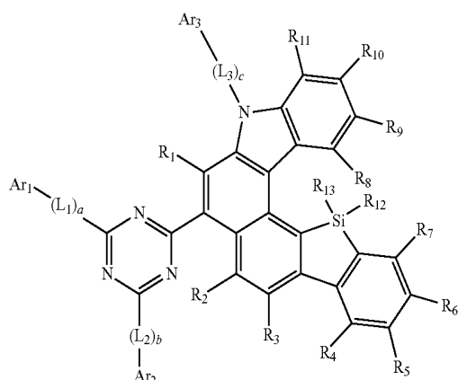
Formula 2c
