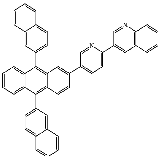
Compound 202
