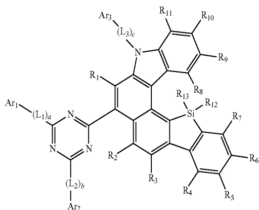
Formula 2f
