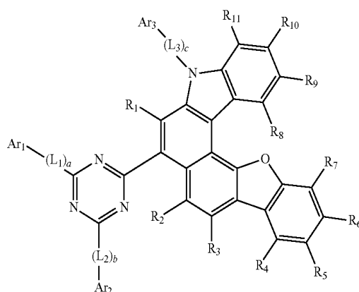
Formula 2c
