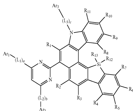
Formula 2f
