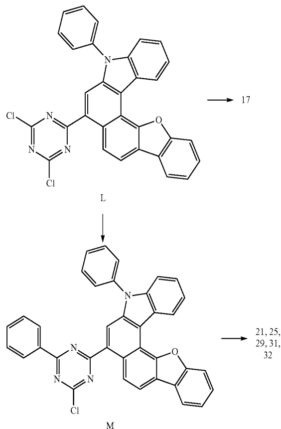
Reaction Scheme 4
