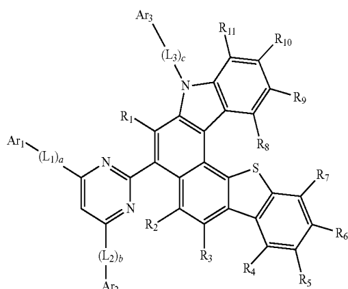
Formula 2d
