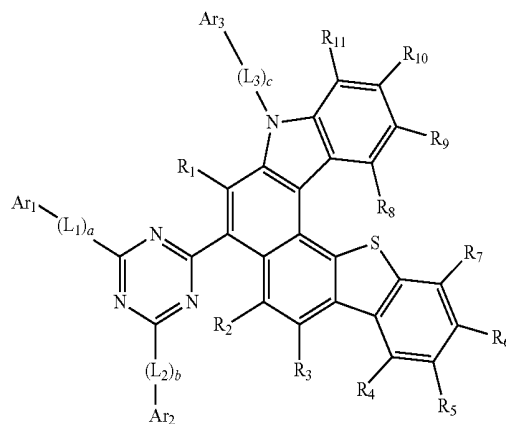
Formula 2a
