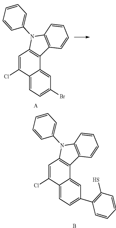
Reaction Scheme 1
