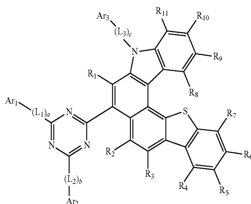
Formula 2b
